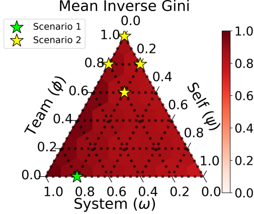
Figure 7: Cleanup : Inverse Gini index for every credo in our evaluation. These experiments have |\mathcal{T}| = 3 teams of two agents each. Despite drastically different rewards, the credos which achieve high rewards also have high equality.
