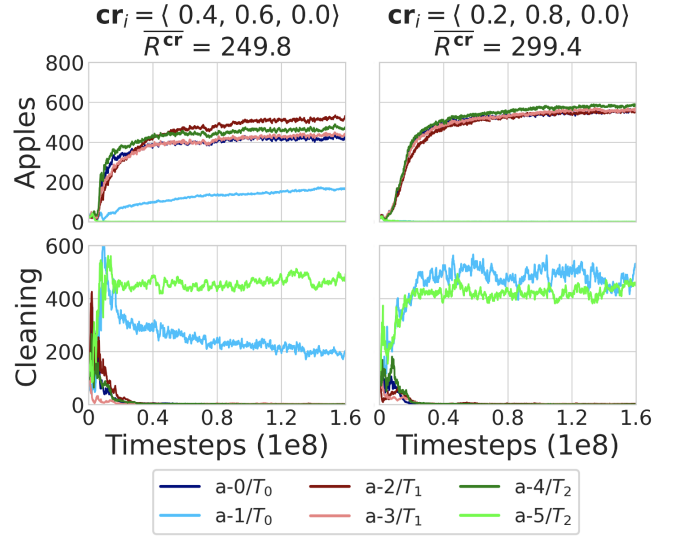
Figure 6: Cleanup: Scenario 2: high team-focus achieves high rewards despite a small amount of self-focus. Each column of plots shows when team-focus is 0.6 (left) and 0.8 (right, a yellow star in Figure 4), offset with self-focus. As team-focus increases, two teams coordinate so at least one teammate cleans the river, leading to better division of labor which is maintained even when agents become fully team-focused.
